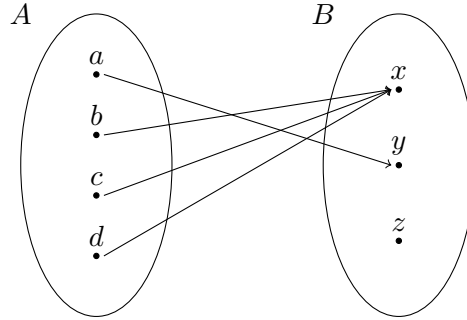
Figure 1.5: Visual representation of the function f : A \rightarrow B .
